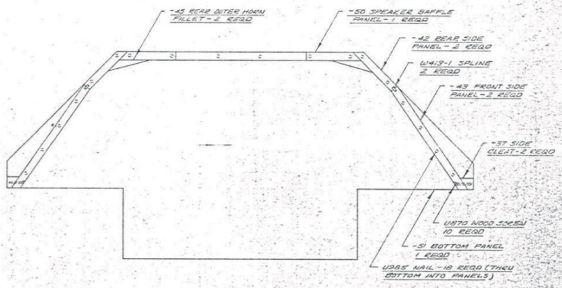
A2 ENCLOSURE SHELL ASSEMBLY - 1 REQD
