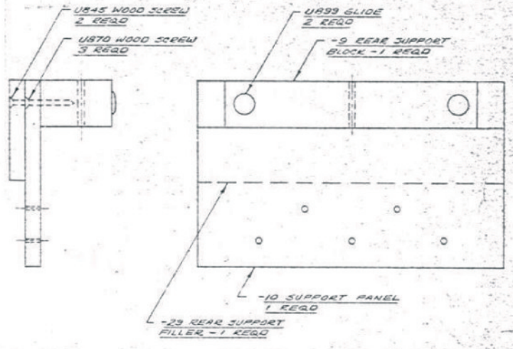
A5 REAR SUPPORT ASSEMBLY 1 REQD \frac{1}{2} SIZE
