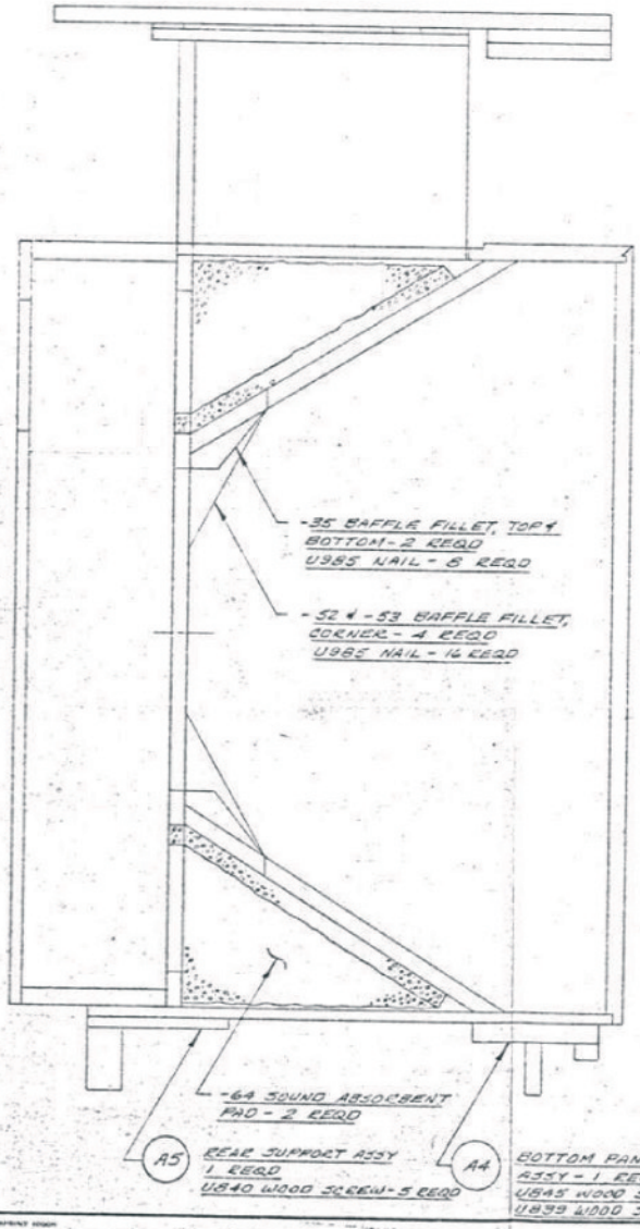
VIEW D-D
