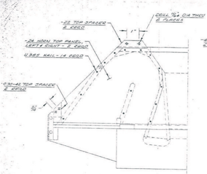
VIEW D-D
